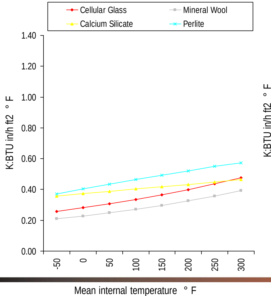
Thermal Conductivity of Insulation Materials Under Ideal Laboratory Conditions (DRY)
