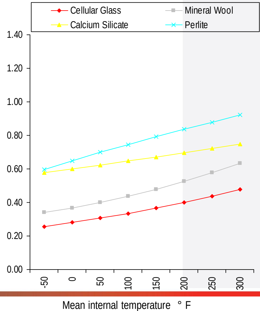
Thermal Conductivity of Insulation Materials with 3% Water Content by Volume
